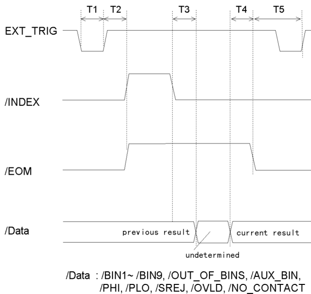
Figure 8. Timing Chart
